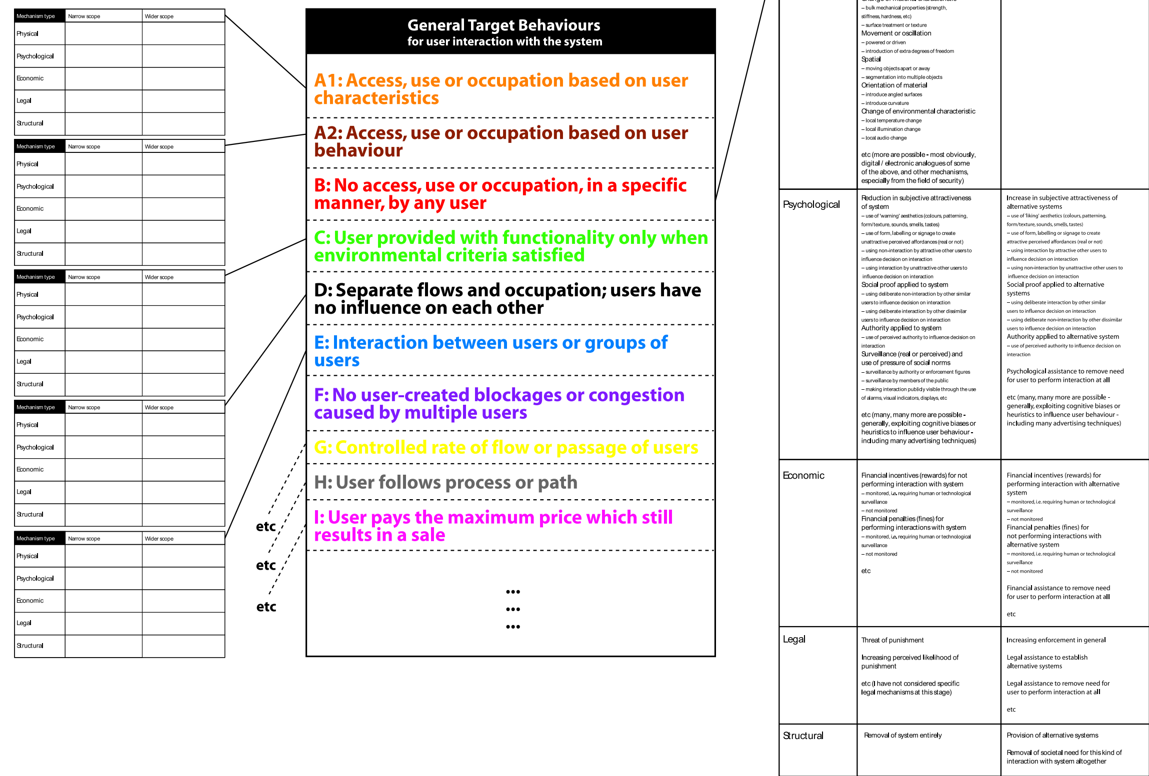
Figure 4.3: The form of DwI v.0.1—a set of general target behaviours and sets of techniques (or ‘mechanisms’), with mappings between them
